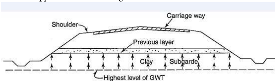
Fig. Capillary cut-off for a clayey subgrade
