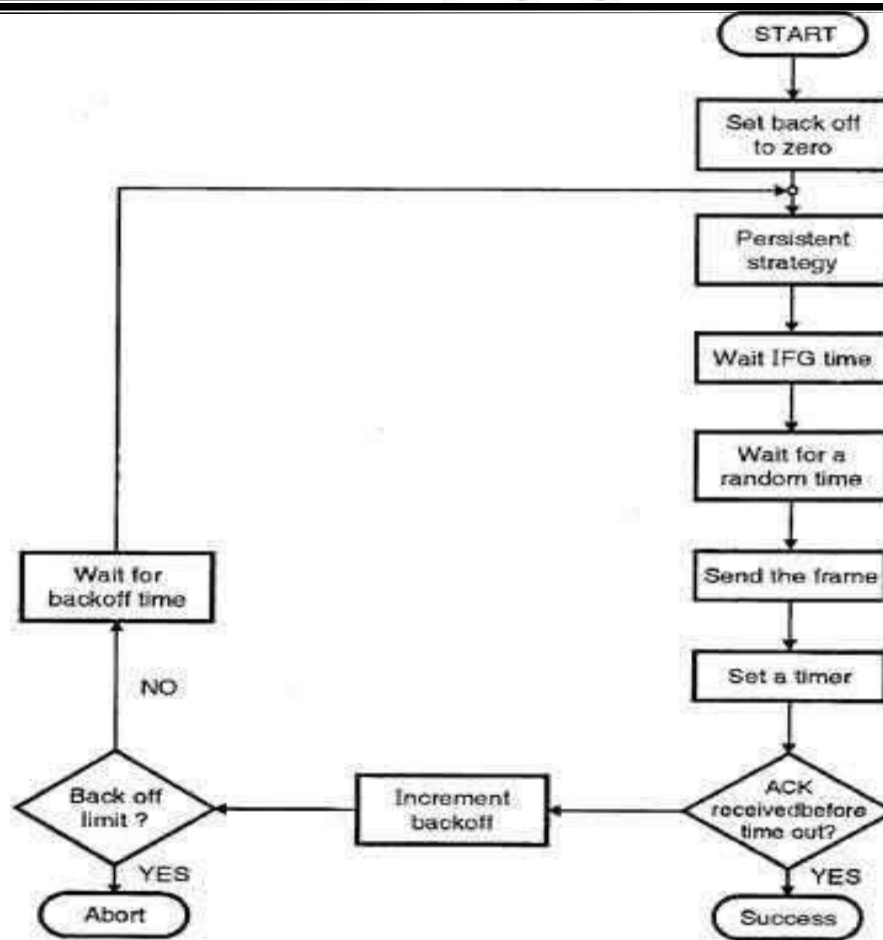
CSMA/CA procedure
