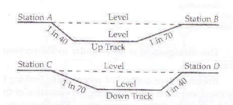
Fig.18 Track Grading
