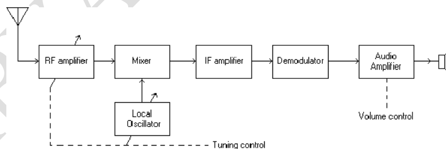
Super-Heterodyne Receiver
