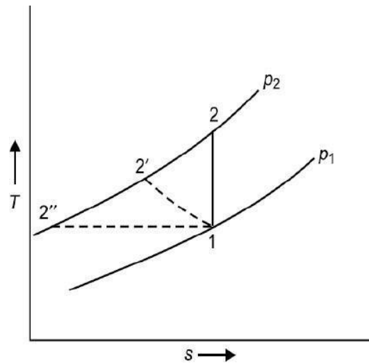
Fig. (3) Compression process on T - S diagram.
