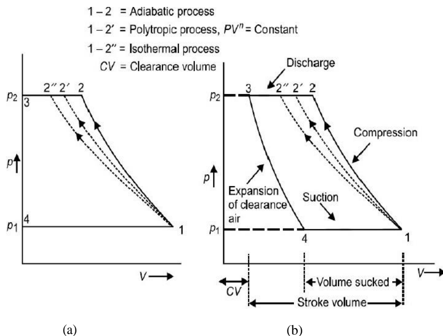
Fig. (2) Compression cycle on p - V diagram (a) without clearance volume (b) with clearance volume
