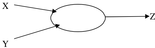
Fig. 4.6 Context Diagram
