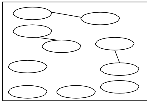
Fig.6.5 Integration Testing
