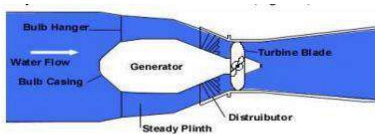
Bulb Turbine
