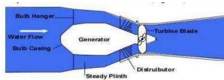
Bulb Turbine
