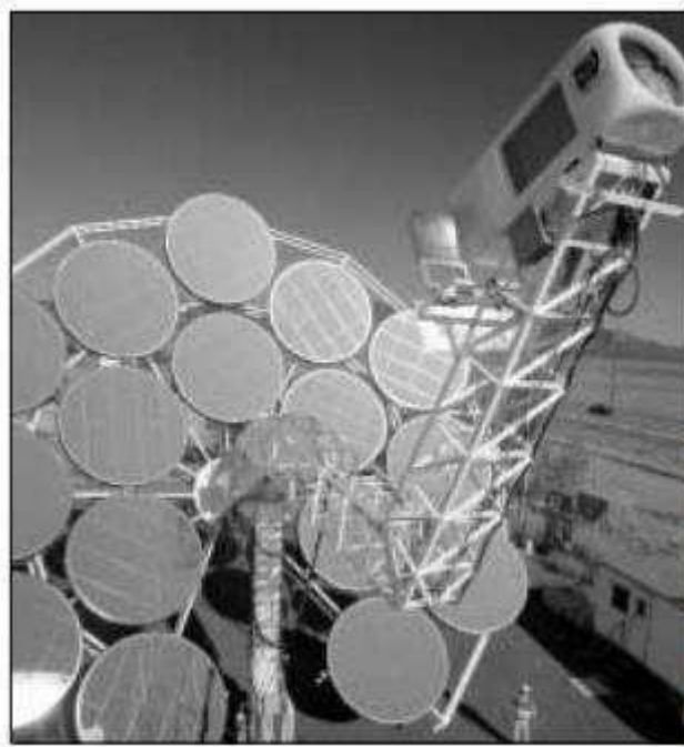
Fig.2 Dish Systems
