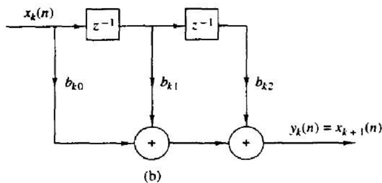
Cascade Realisation of a FIR system
