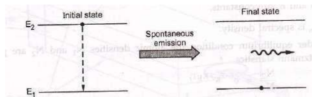
Fig. 3.1.8 Spontaneous emission
