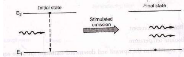
Fig. 3.1.9 Stimulated emission
