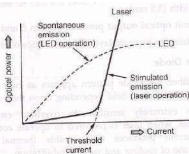
Fig. 3.1.13 Optical characteristics of an LED and laser compared
