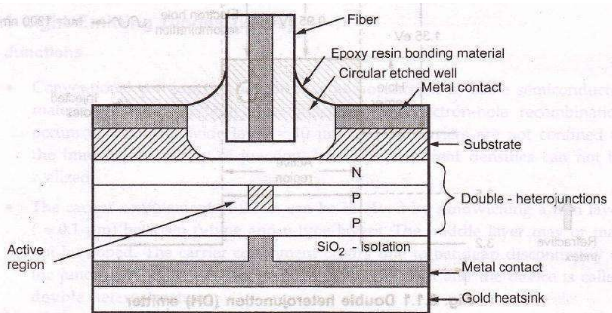
Fig. 3.1.2 Cross-section through a typical surface emitting LED
