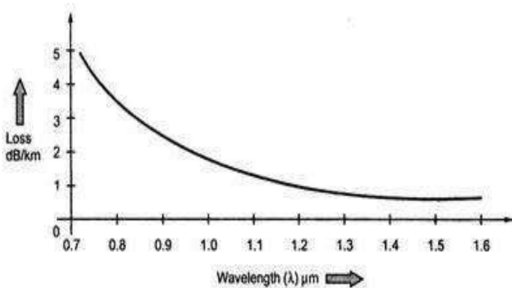
Fig. 1 Scattering loss
