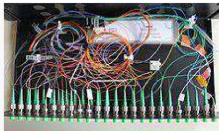
WDM multiplexer for DWDM communications
